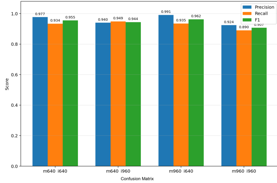
Confusion Matrix
